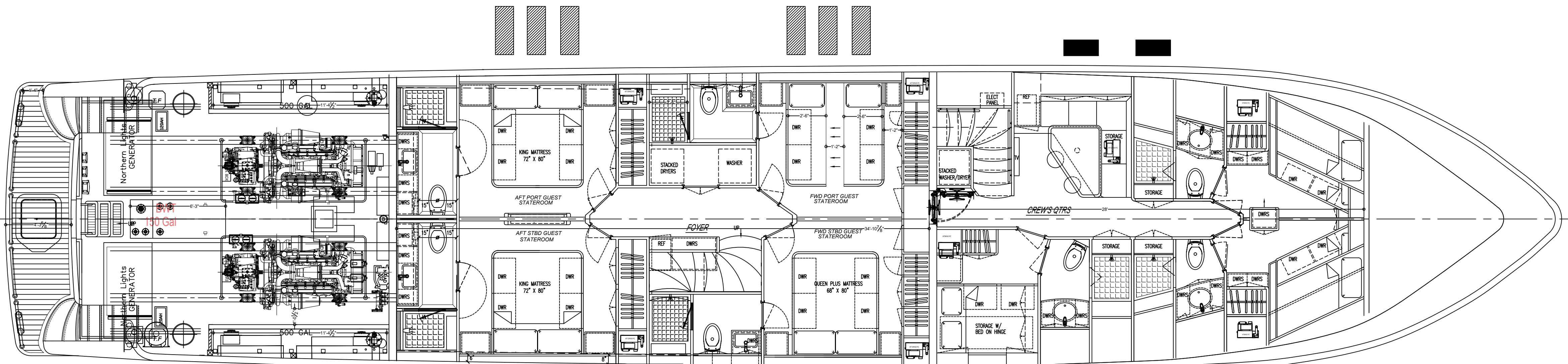
LOWER DECK
